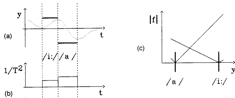
Fig. 1: Tongue body movement and gestural targets (bold horizontal bars) for successive /i:/ and /a/ gestures (a), rectangular force functions within the activation interval (b) and resulting force fields depending on distance from target position (c; thick vertical bars equalling horizontal ones in (a); after Kröger et al. 1995: 1880).
