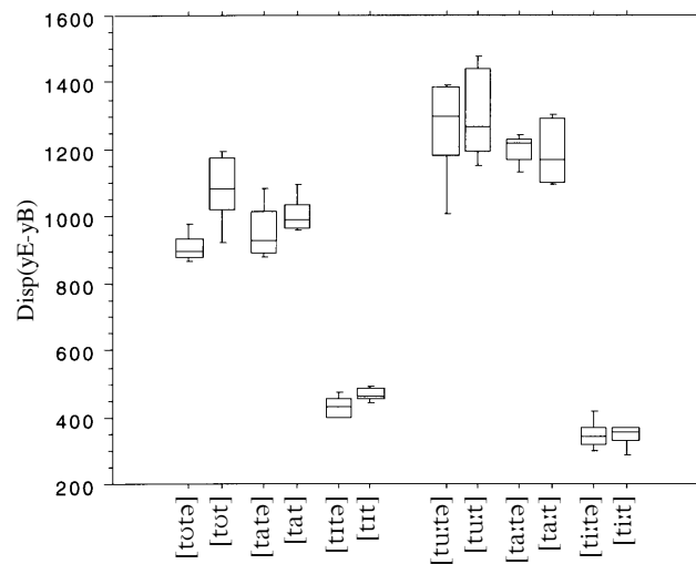
Fig. 14: Displacement (Disp(yE-yB)) of the tongue tip coil during the [t] closure gesture (values are given in 10 -2 mm).
