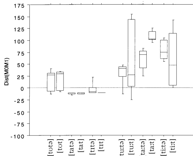
Fig. 35: Temporal distance between the end of the vocalic opening gesture and the beginning of the [t] closing gesture (in ms).
