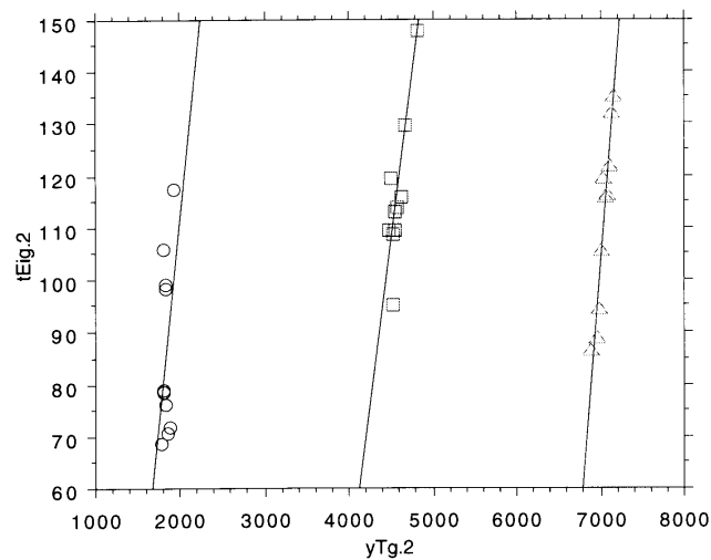
Fig. 27: Scatterplot of target position vs. eigenperiod value of the [t] closing gesture for the lax vowels with the calculated regression lines shown superimposed (circles: [ɔ], r = .397 , n.s.; squares: [a], r = .849 ; triangles: [ɪ], r = .964 ).
