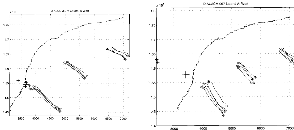
Fig. 34: Comparison of the trajectories and gestural target positions between lax [a] (left) and tense [a:] (right) vowel contexts for the lateral closing gesture.
