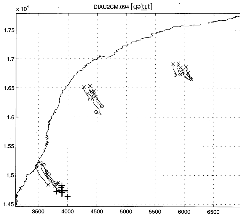
Fig. 29: Articulatory trajectories of the vocalic opening gestures in [gə'tɪt] as delimited in the kinematic analysis of the tongue tip coil (o marking measured movement onset, x movement offset) superimposed along with the palate tracking and the model derived gestural target positions (crosses) and the mean target location (large cross).
