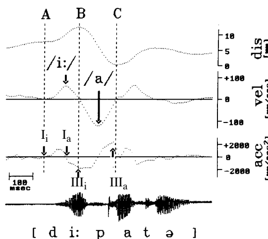
Fig. 4: Starting values of the fit algorithm for the successive /i:/ and /a/ gestures of fig. 3 (see text for details; after Kröger et al. 1995: 1883).
