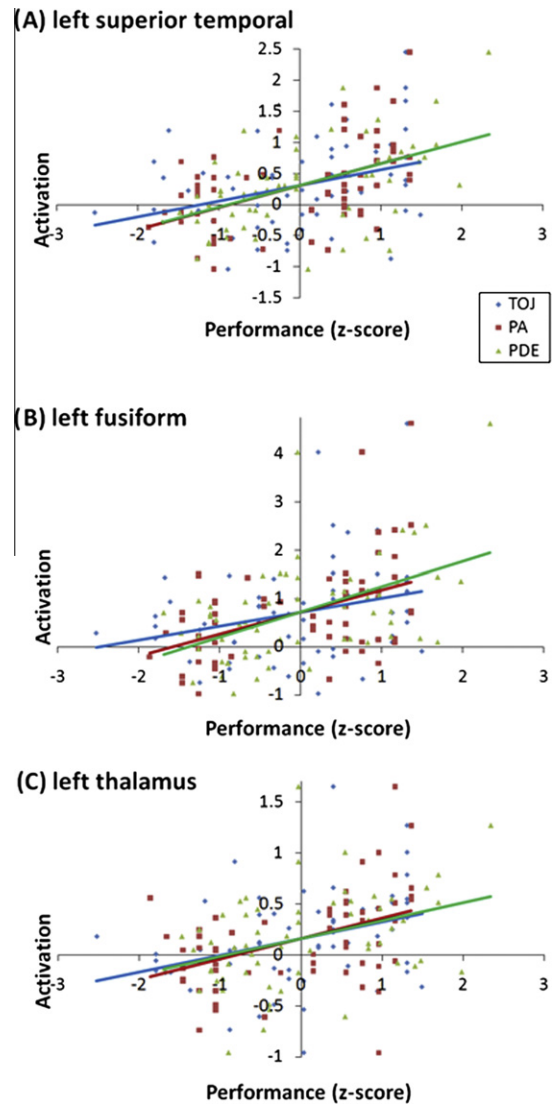
Fig. 3. Scatterplots and regression lines showing correlations of rapid temporal order judgment (blue), elision (red), and phonemic decoding efficiency (green) measures with standardized activation values for print in the left superior temporal gyrus (A), left fusiform gyrus (B), and left thalamus (C).
