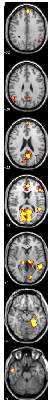
Fig. 2. Areas showing a correlation between activation levels for print (words and pseudowords) and component scores reflecting shared variance among behavioral predictors of reading skill. Images are presented in radiological convention with the left hemisphere on the right side of the images at a univariate threshold of p < 0.01 , corrected for mapwise false discovery rate (FDR; Genovese, Lazar, & Nichols, 2002 ) with a cluster threshold of 10 contiguous significant voxels. Numbers of the lower left side of each slice corresponds to the position along the Z-axis in MNI space.
